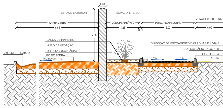
PORMENOR P01
